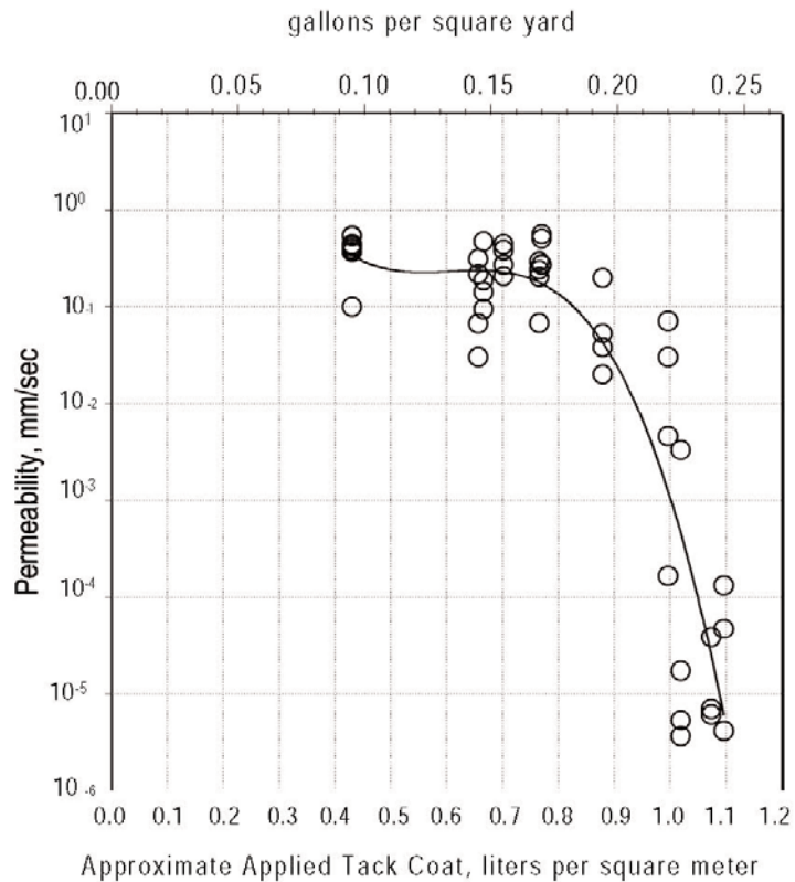
Figure 1 - Results of permeability tests on paving fabric specimens cut from melt through asphalt absorption tests. The asphalt quantity is the amount absorbed by the paving fabric plus the required 0.23 l/m 2 (0.05 gal/yd 2 ) for interlayer system bonding.
